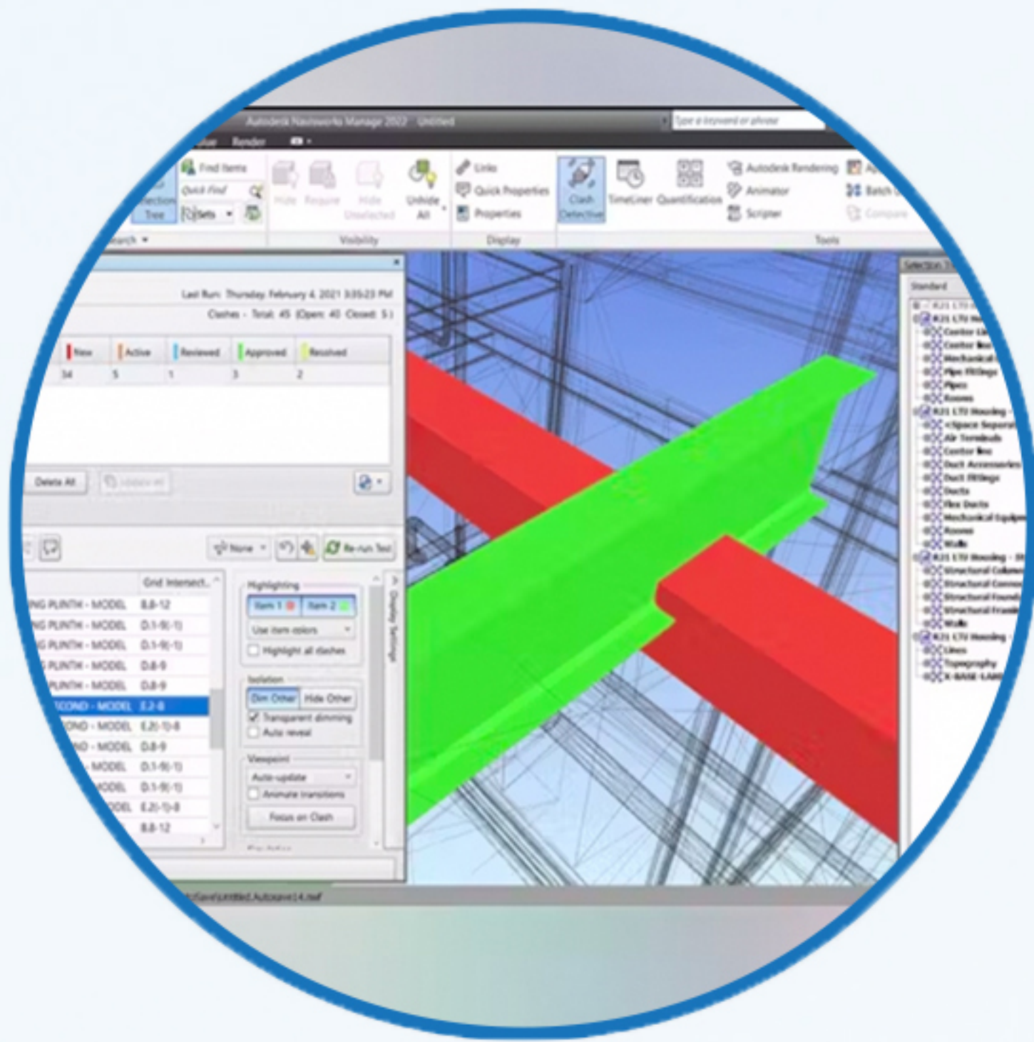
Clash Detection between services
